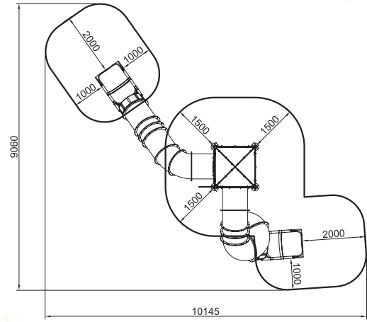
LD202.01 TORRE CASTILLO (1T+2T)
