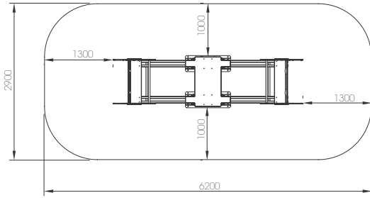
LD109.08 BALANCIN COHETE
