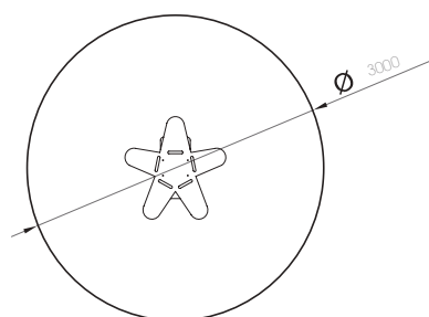
LD107.01 MUELLE QUINTUPLE STAR
