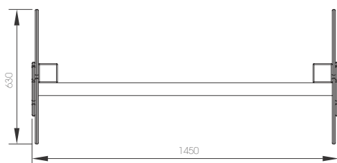
LC012.01 VALLA HUESO SALTO REGULABLE
